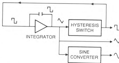
Basic Function Generator
