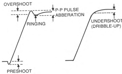
Waveform Distortion
