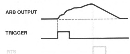
Triggered Arb with Ramp-to-Start
