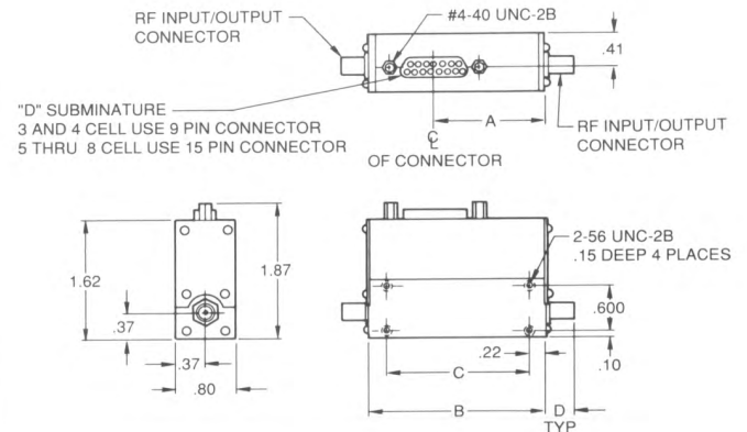
DIMENSIONS (INCHES)
