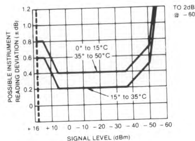
Figure 1. Models 1038-N10 System Coaxial Detector Accuracy from 1 MHz to 26.5GHz.
