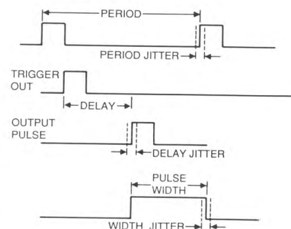
Period, Delay & Width Jitter
