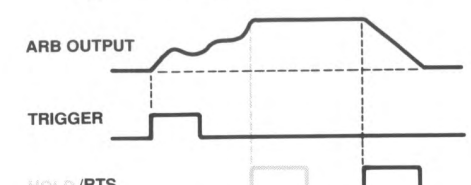
Triggered Arb with Hold and Triggered Ramp-to-Start
