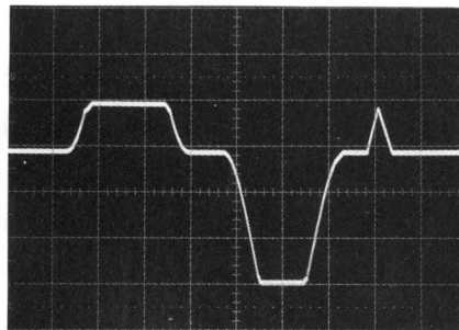
Typical Disk Sync Waveform
