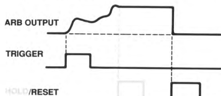
Triggered Arb with Hold and Triggered Reset
