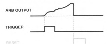
Triggered Arb with Reset
