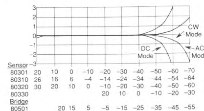
Linearity Plus Zero Set vs. Input Power
