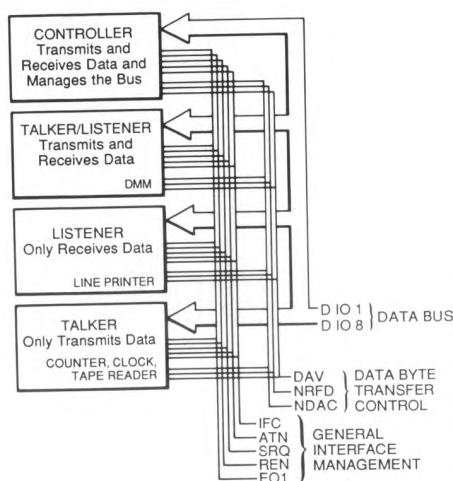
Figure 1. Types of Instruments on the Bus.
