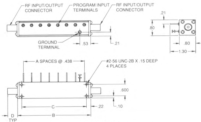
DIMENSIONS (INCHES)
